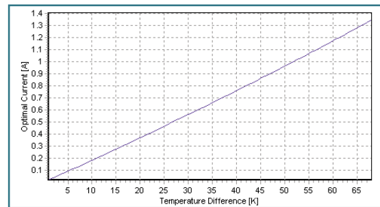
Figure 5.5.3. I_{opt}(\Delta T)
