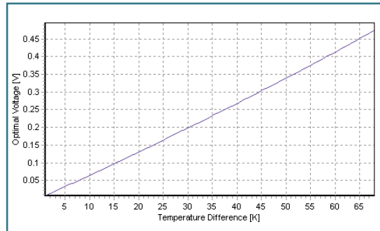
Figure 5.5.5. U_{opt}(\Delta T)
