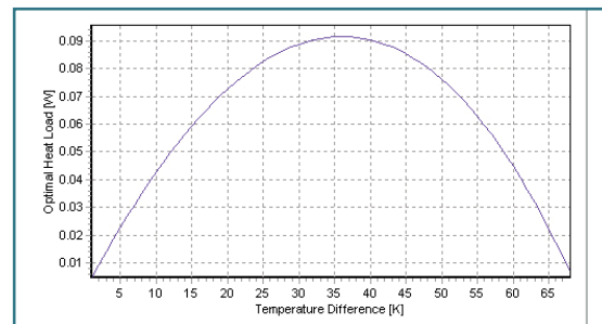
Figure 5.5.4. Q_{opt}(\Delta T)
