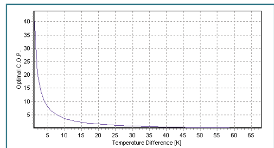
Figure 5.5.2. COP_{opt}(\Delta T)
