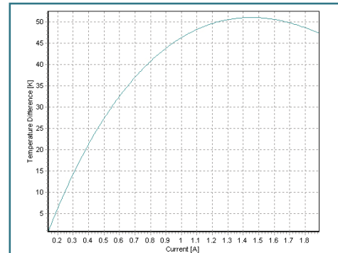
Figure 5.6.1. \Delta T(I) at a the summed heat load Q
