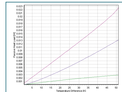
Figure 5.6.4. Passive heat loads of different nature: radiation, convection, thermal conduction
