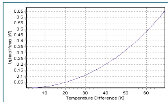
Figure 5.5.6. P_{opt}(\Delta T)
