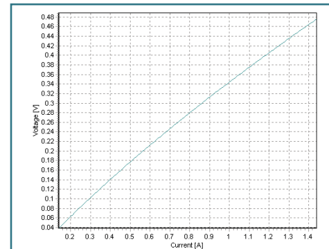
Figure 5.6.2. U(I) at a the summed heat load Q
