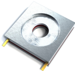
Customized TEC plates thickness & machining
