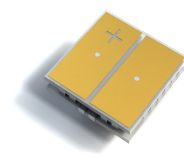
SMD / Flip-chip (contacts on hot side)
